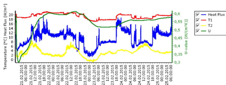
Figure 1: Results of heat flux measurement (Report on basis of greenTEG Software v1.00.03. 2015)
