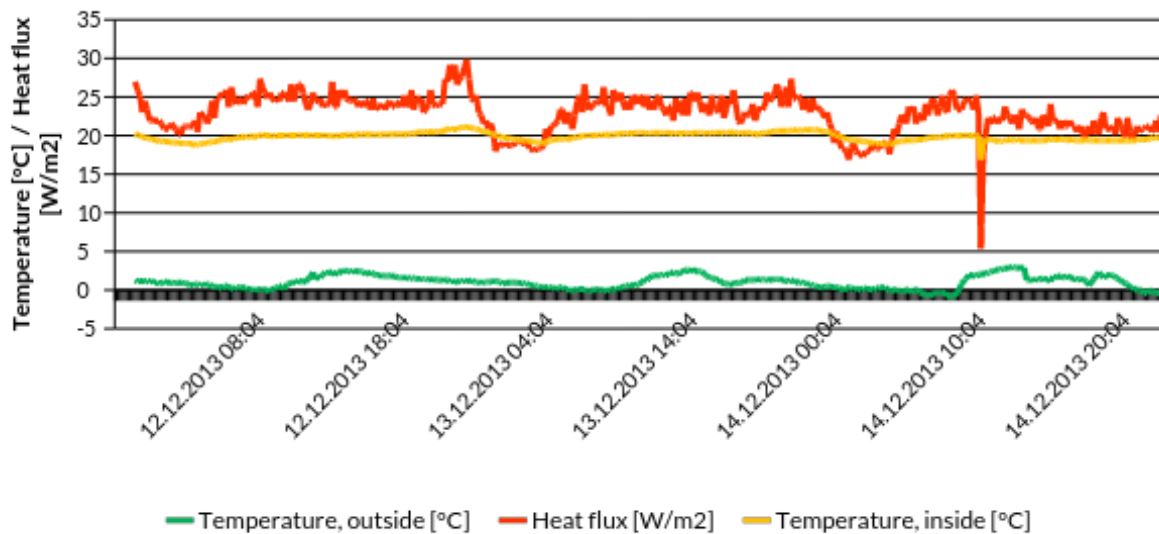
Figure 4. Temperature and heat flux of spot A. This graph was created using the (old) software included in the measurement device (new software version shows directly U-value graph).
