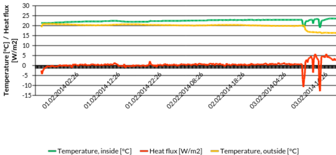
Figure 5. Temperature and heat flux graph of spot B. The outside temperature corresponds to the temperature in the cellar. This graph was created using the (old) software included in the measurement device (new software version shows directly U-value graph).
